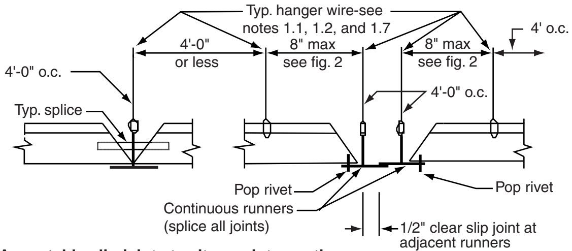
(A) Acceptable slip joint at exitways intersection
