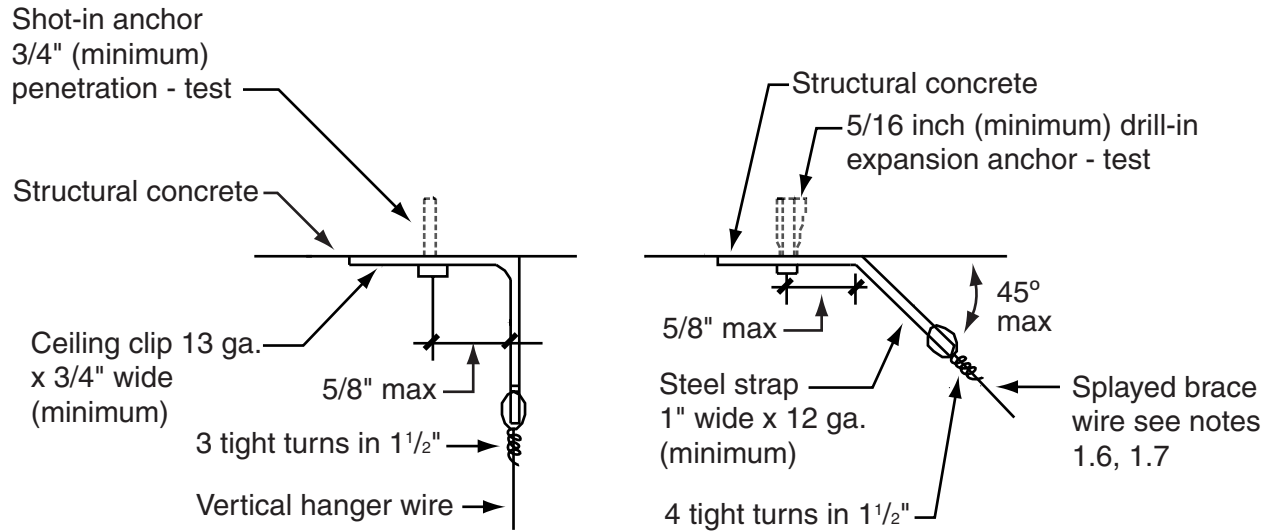
(A) Vertical hanger wire clip attachment (B) Splayed bracing wire clip attachment
